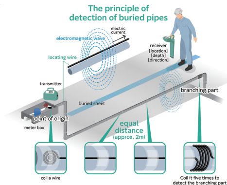
Construction drawing of locating wire
