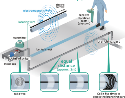
Construction drawing of locating wire
